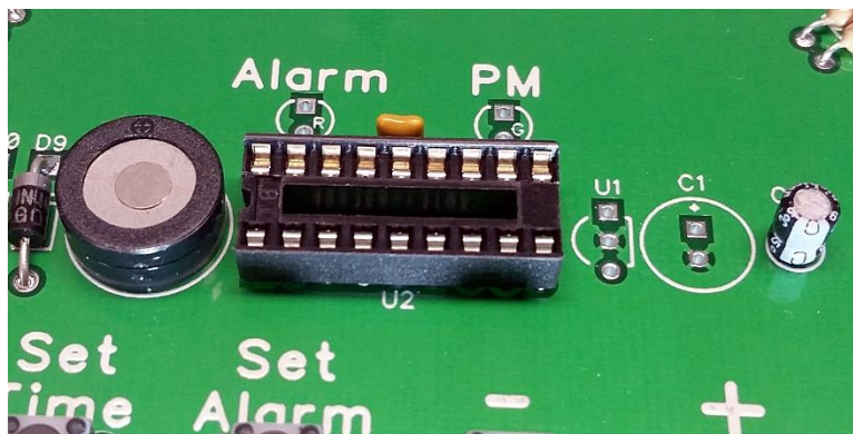
Figure 18 – BZ1 and C2 installed – note their orientation
