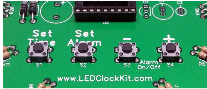
Figure 15 - Pushbuttons installed
