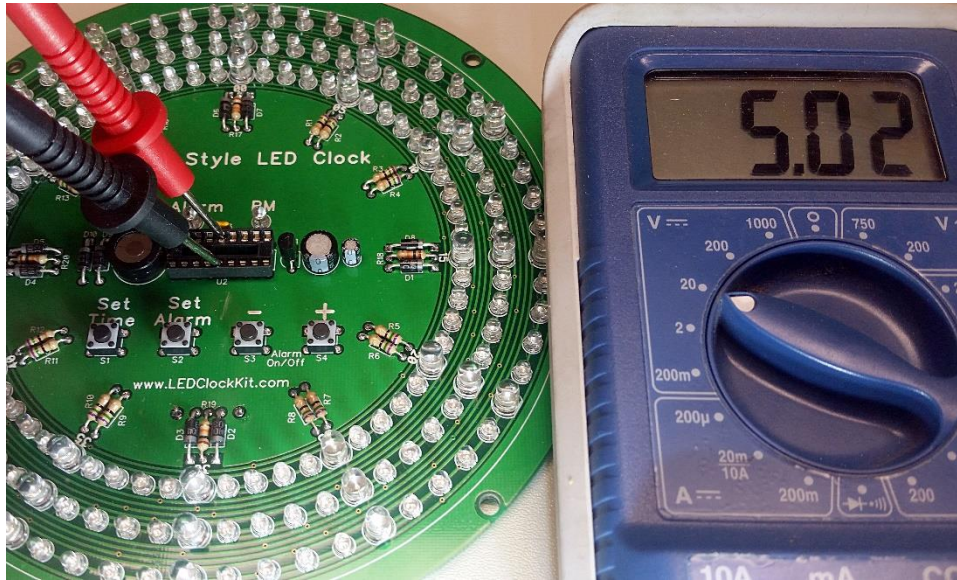
Figure 38 – Checking the power supply to U2
