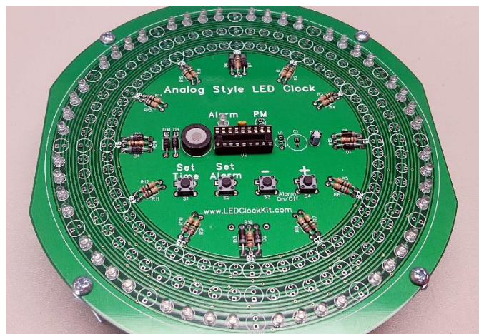
Figure 26 – All 3mm Red LEDs installed
