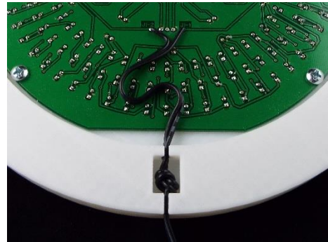
Figure 42 – Routing the power cord
