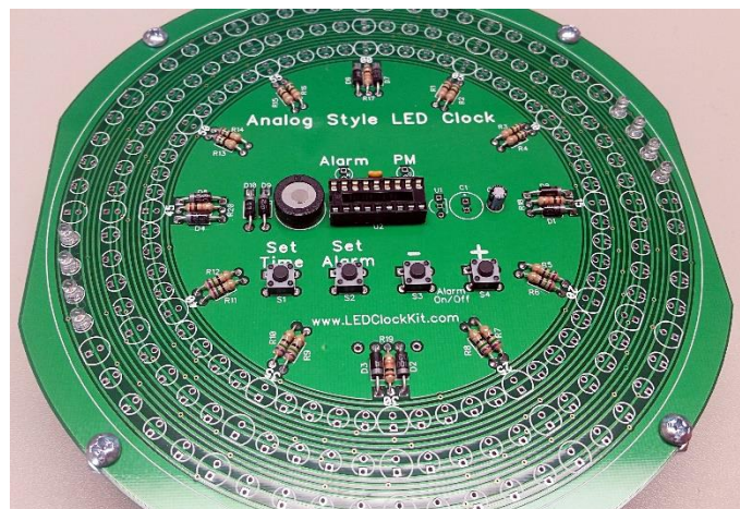
Figure 25 – Inserting LEDs eight at a time
