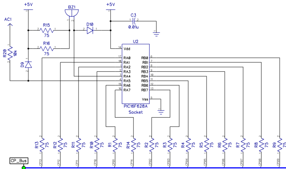
Figure 50 – Schematic, Microcontroller
