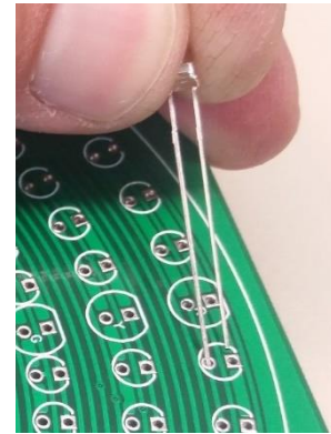
Figure 24 Proper LED orientation
